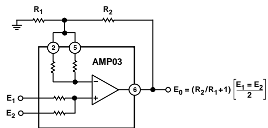
Figure 26. Precision Summing Amplifier with Gain
